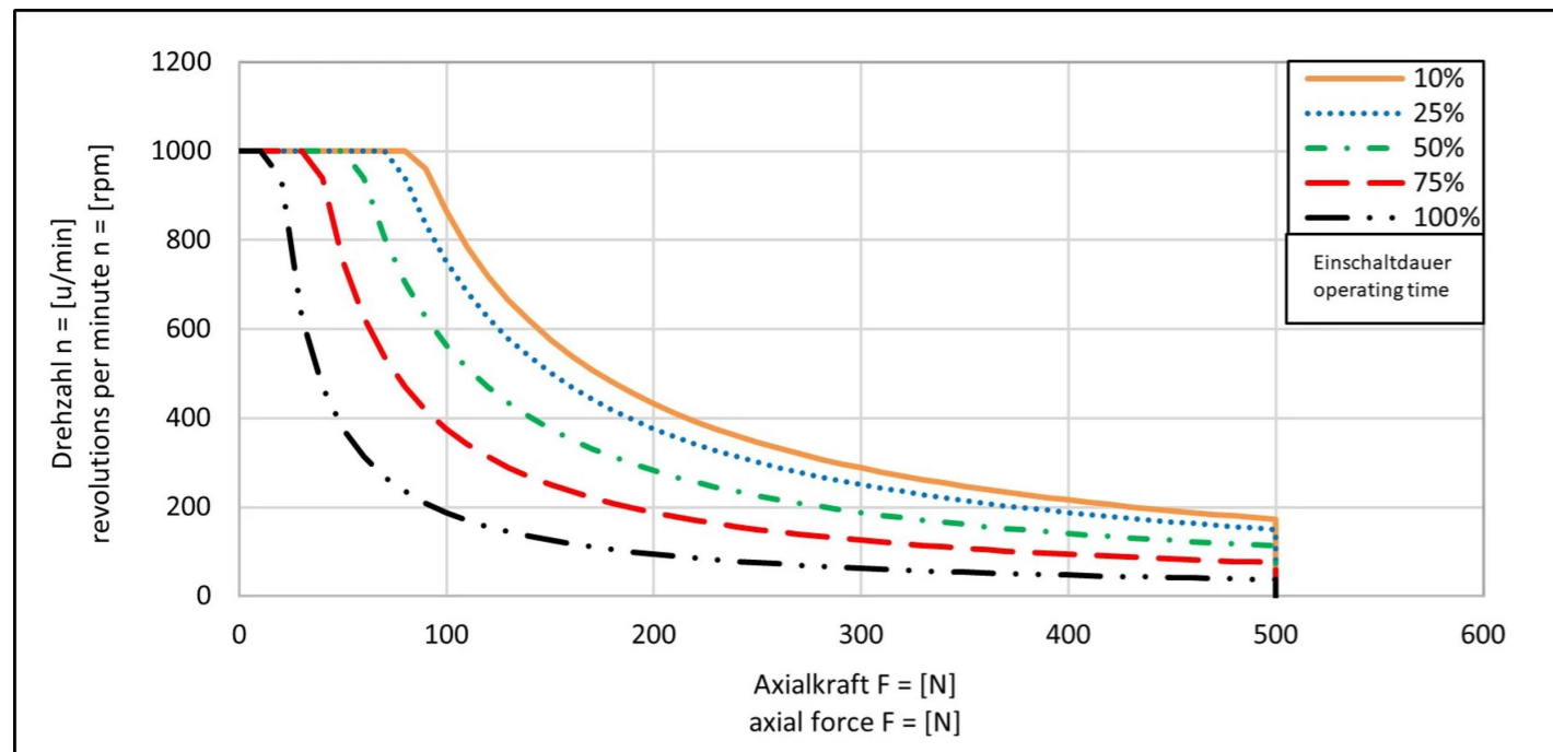
Diagram 1: Stroke / speed
