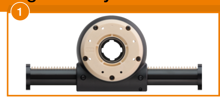
drygear® Apero® cantilever axis configurable in different lengths with coupling half with a diameter of 8mm
