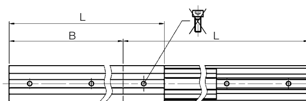
Partial extension NT-35-"L"-"B"
